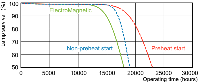
TL-D Super 80 Life Expectancy 12 h cycle
